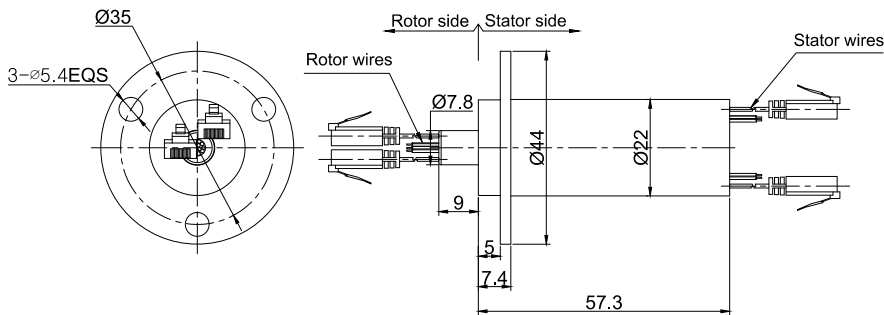
BXME1222-S18 Outline dimension drawing
