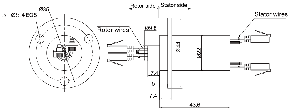
BXME1222-S06 Outline dimension drawing
